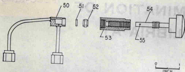
Figure 2. Liquid sampler
