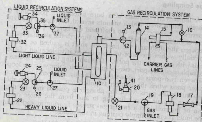
Figure 4. Gas and liquid recirculation systems
