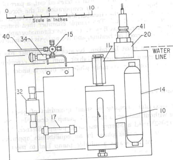
Figure 1. Elevation view of major components
